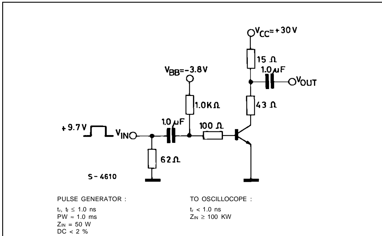
Test Circuit for t_{on} , t_{off} .
